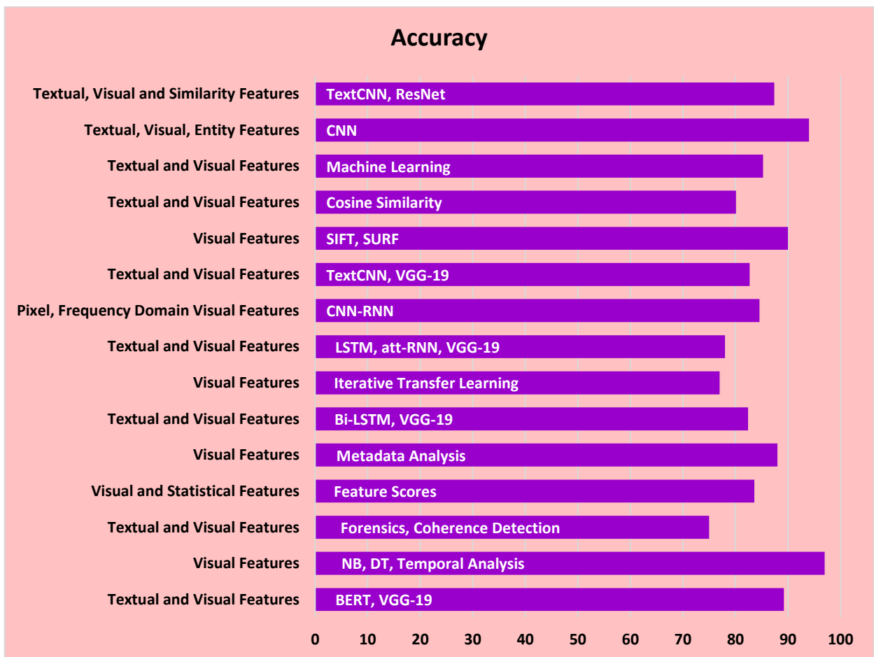
Figure 18: Performance comparison based on accuracy scores
